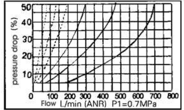
Characteristic Curve Of Flow Rate
