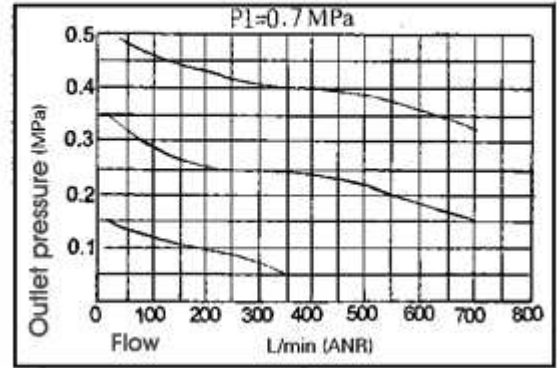
Characteristic Curve Of Flow Rate
